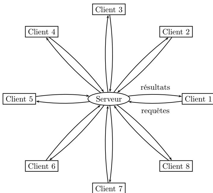
FIGURE 10.1 – Architecture client-serveur
