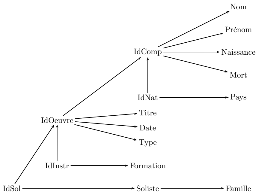
FIGURE 10.9 – Graphe ADF
