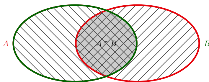
FIGURE 2.1 – Intersection de deux ensembles
